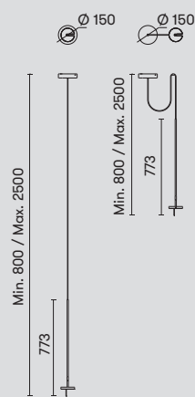
Touch dimmer
